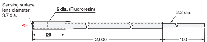
E32-T51F (R40) Free-cut
