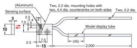
15-G E32-D15ZR 2M (Free Cutting)
