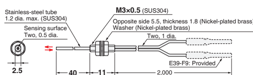
19-I E32-D22-S1 2M (Free Cutting)
