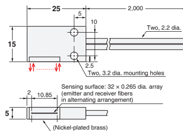
49-E E32-D36P1 2M (Free Cutting)
