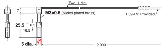
21-C E32-C31N 2M (Free Cutting) + E39-F3A-5
