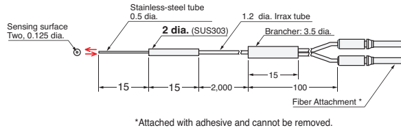
17-H E32-D33 2M (Free Cutting)
