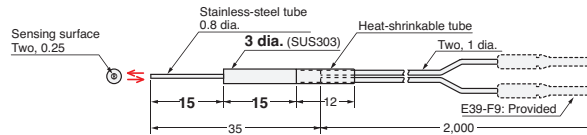
17-I E32-DC200F4R 2M (Free Cutting)
