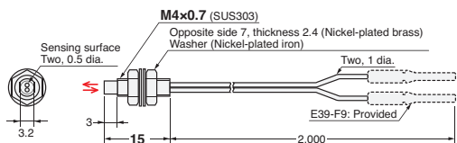
41-D E32-D21B 2M (Free Cutting)
