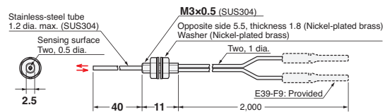
17-I E32-DC200F4R 2M (Free Cutting)
