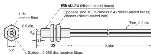
09-H E32-CC200 2M (Free Cutting)
