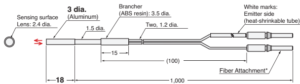
19-E E32-C42S 1M (No Cutting)
