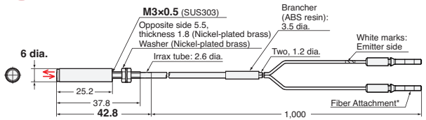
21-D E32-C41 1M (No Cutting) + E39-F3B
