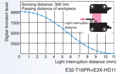
Characteristics of Light Interruption (Typical)
