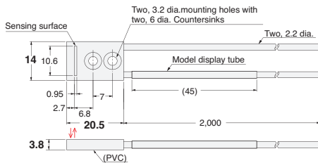
35-B E32-L16-N 2M (Free Cutting)
