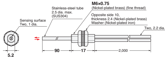
17-J E32-DC200BR 2M (Free Cutting)
