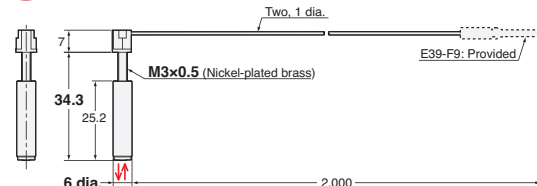
21-F E32-C31N 2M (Free Cutting) + E39-F3B
