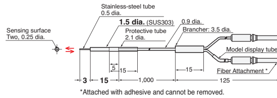
17-G E32-D331 2M (No Cutting)
