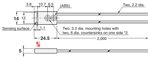
53-C E32-A08H2 3M (No Cutting)
