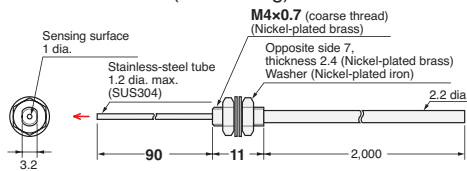
17-D E32-TC200BR 2M (Free Cutting)
