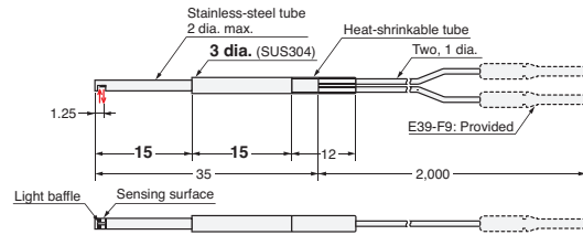
17-E E32-D24R 2M (Free Cutting)
