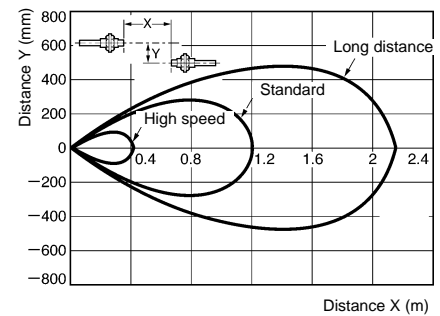
E32-T11 (Through-beam)
