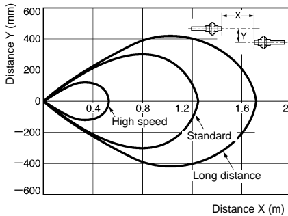
E32-TC200 (Through-beam)
