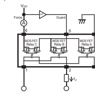
Example of G3VM-21MT measuring circuit
