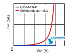
Current leakage I LEAK vs Applied voltage V DD
