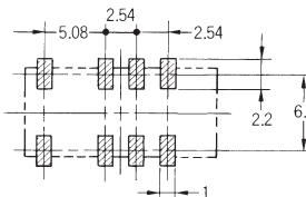
Footprint (Bottom View)
