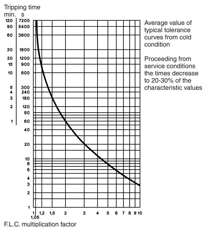
with three-phase load
