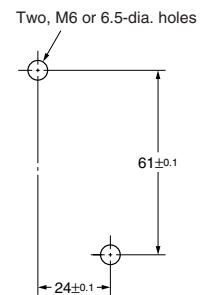
Mounting Hole Dimensions (TOP VIEW)
