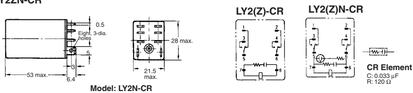
Terminal Arrangement/Internal Connections (Bottom View)
