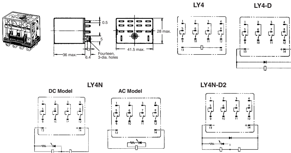
Terminal Arrangement/Internal Connections (Bottom View)
