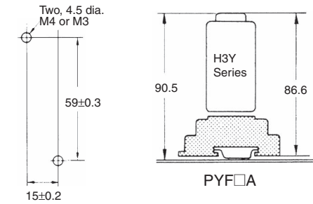
Mounting Holes
