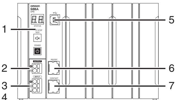
S8BA-24D24D240LF (240 W)
