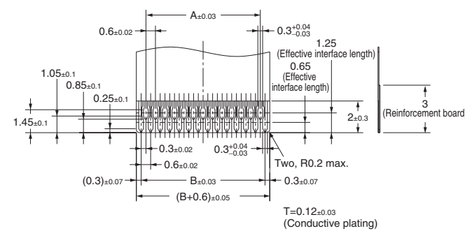
Applicable FPC Dimensions
