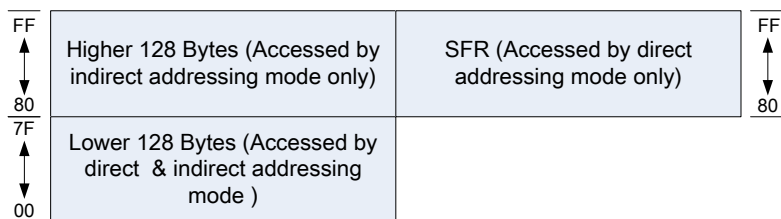
图 3-2: RAM architecture
