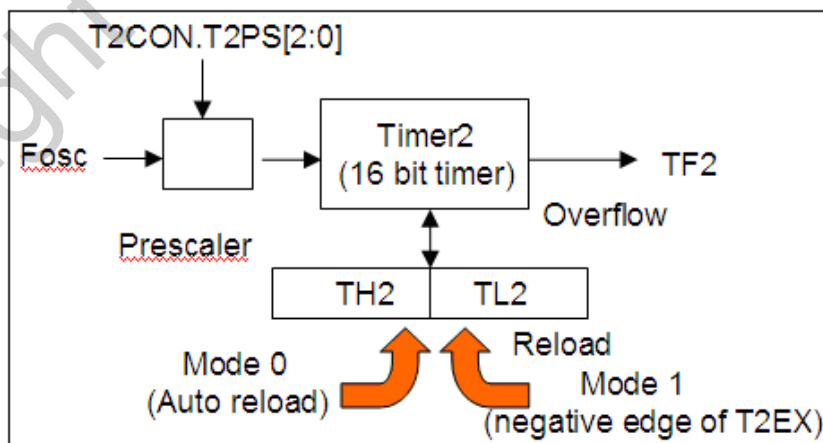
图 7-1: Timer mode and Reload mode function
