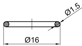
Seal Ring
