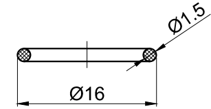
Seal Ring
