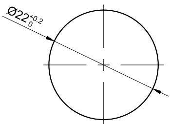
PANEL CUTOUT MAX.PANEL THICKNESS 8 mm
