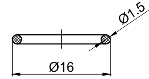
Seal Ring
