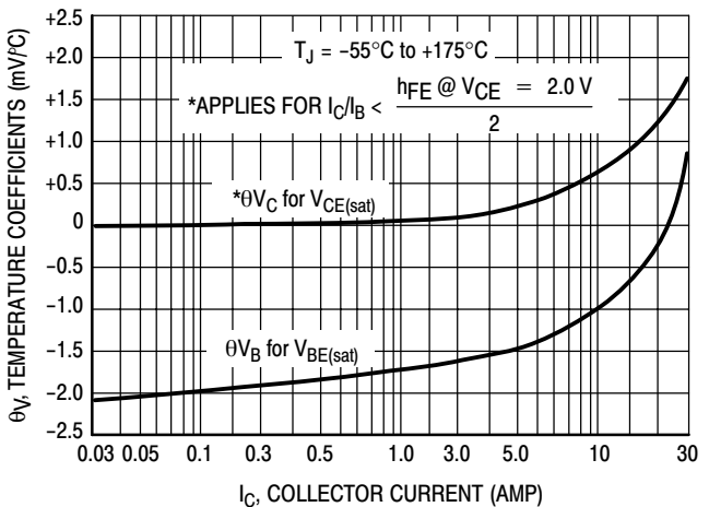
Figure 14. Temperature Coefficients
