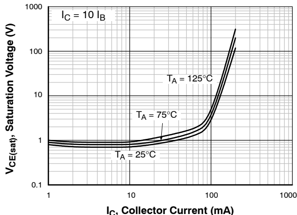
Figure 2. Saturation Voltage
