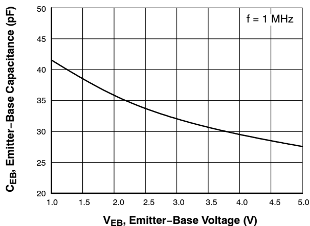
Figure 8. Input Capacitance
