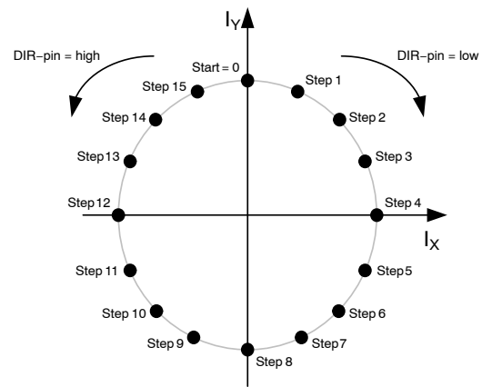
Figure 13. 1/4 Microstepping
