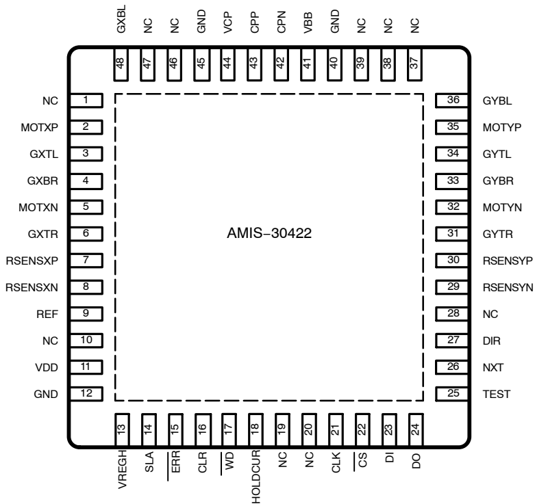
Figure 2. Pin Out AMIS-30422
