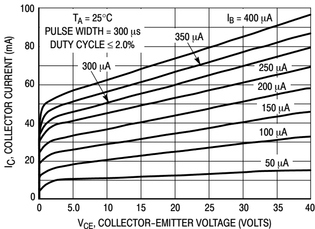
Figure 7. Collector Characteristics
