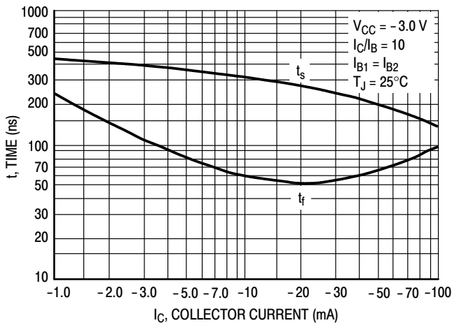
Figure 11. Turn-Off Time
