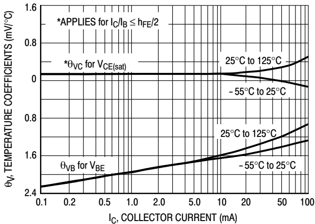
Figure 9. Temperature Coefficients
