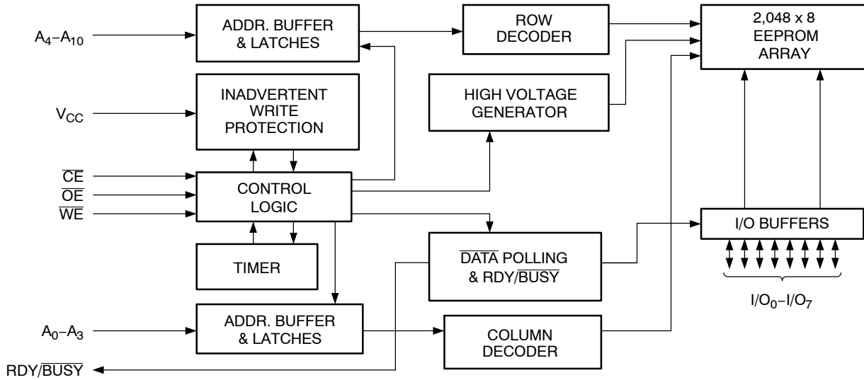
Figure 1. Block Diagram
