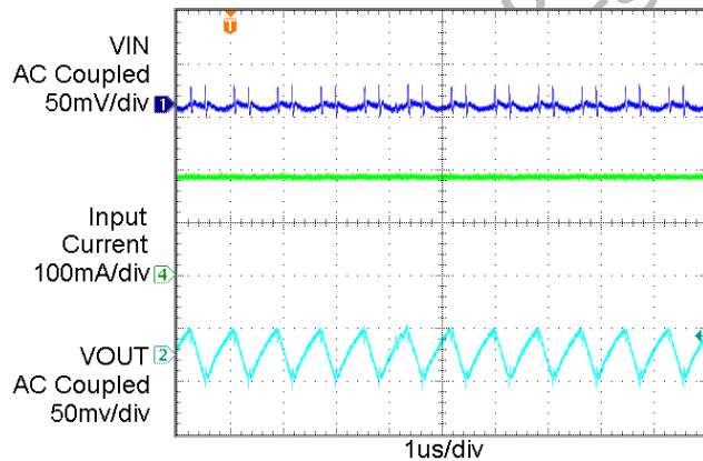
Figure 20. Switching Waveforms in 1.5x Mode
