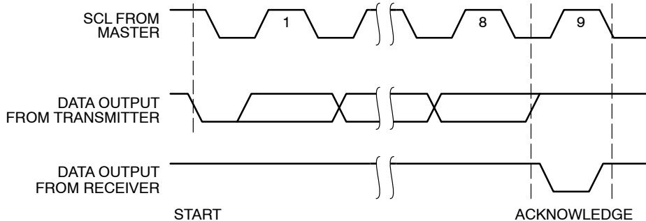
Figure 5. Acknowledge Timing
