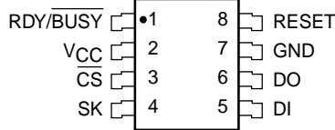
SOIC Package (S, V)
