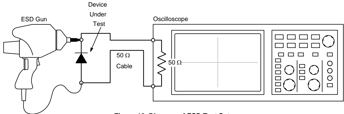
Figure 12. Diagram of ESD Test Setup
