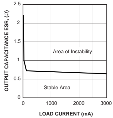
Figure 11. Stability Region VIN/VOUT = 5V/1.5V
