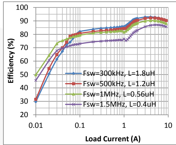
Figure 6. FAN2306A Efficiency vs. Load Current with V_{IN}=12\text{ V} and V_{OUT}=1.2\text{ V}
