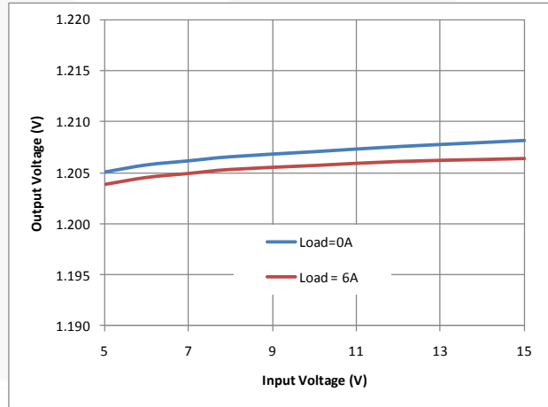
Figure 14. Line Regulation
