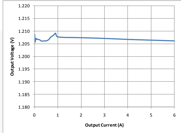
Figure 12. Load Regulation
