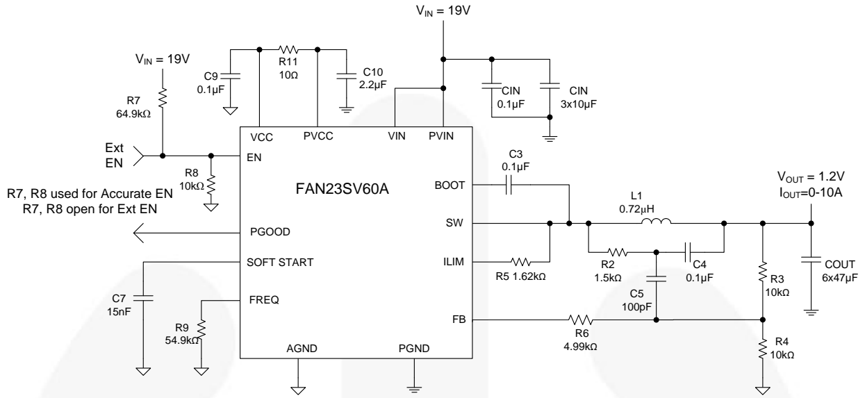
Figure 1. Typical Application with V_{IN} = 19\text{ V}
