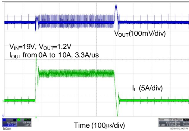
Figure 24. Load Transient from 0% to 50% Load Current
