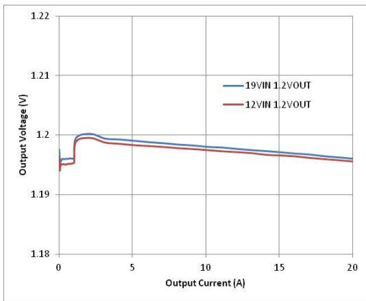
Figure 14. Load Regulation
