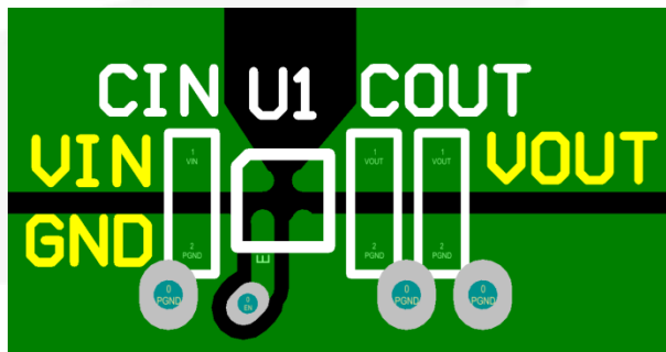
Figure 18. Recommended Layout
