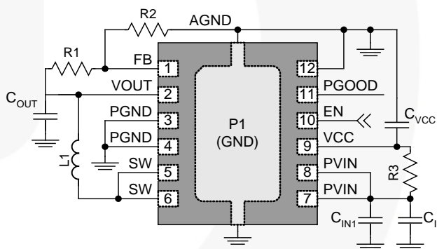
Figure 1. Typical Application
