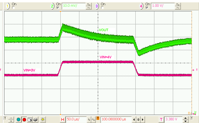
Figure 21. Line Transient, I_{LOAD}=1.0\text{ A} , t_r=t_f=10\ \mu\text{s}
