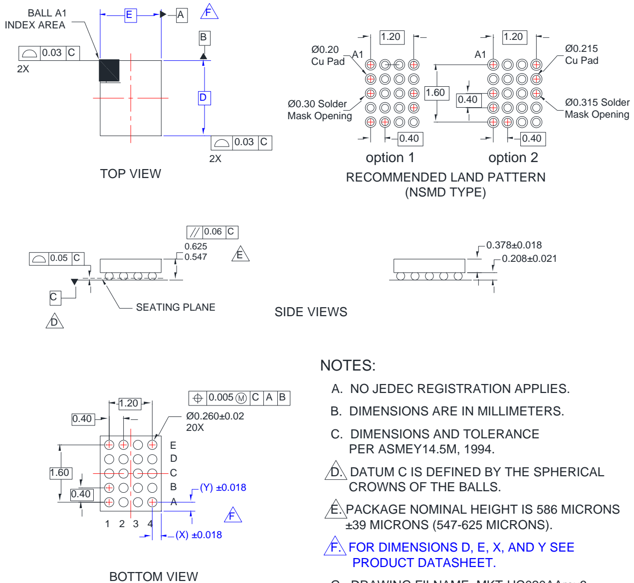
Figure 31 20-Ball WLCSP, 4x5 Array, 0.4mm Pitch, 250 μm Ball
