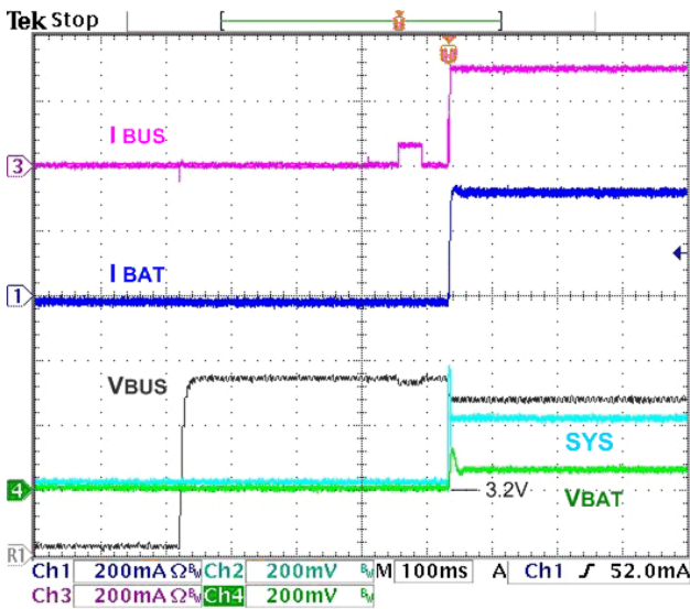
Figure 13. Charger Startup at V_{\text{BUS}} Plug-In Using 300 mA Current Limited Source, 500 mA I_{\text{BUSLIM}} , 3.2 V_{\text{BAT}} , 50 \Omega SYS Load
