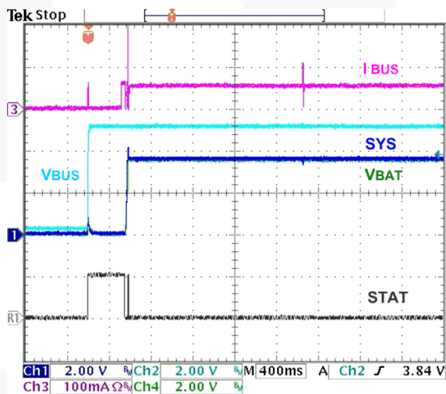
Figure 18. No Battery at V_{BUS} Power-Up, FAN54042, 100\ \Omega SYS Load, 1\text{ k}\Omega V_{BAT} Load
