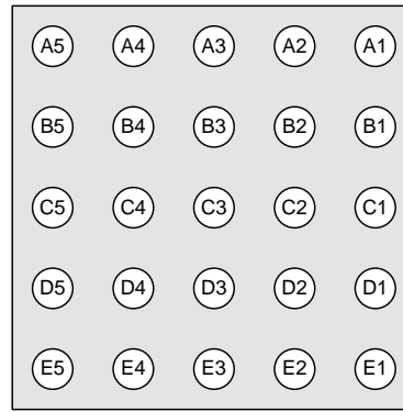
Figure 4. Bottom View
