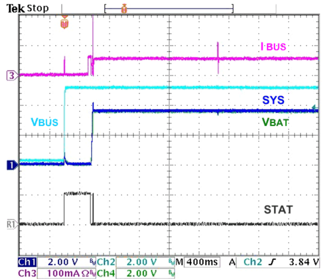
Figure 20. No Battery at V_{BUS} Power-Up, 100\ \Omega\text{ SYS Load} , 1\text{ k}\Omega\text{ V}_{BAT} Load
