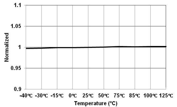
Figure 9 Ratio between V_{LPC} & V_{RES} ( Ratio_{LPC-RES} ) vs. Temperature
