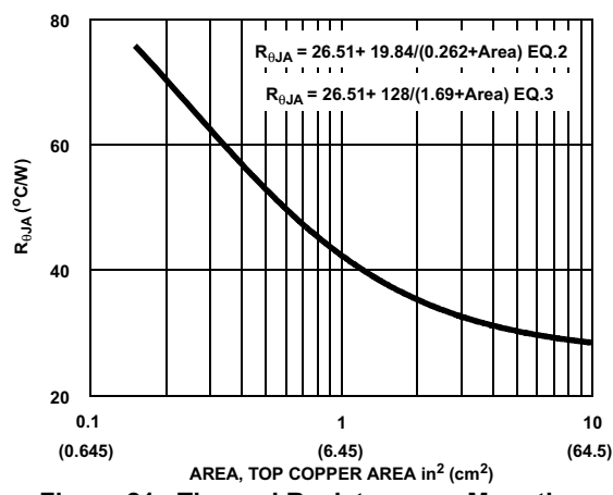
Figure 21. Thermal Resistance vs Mounting Pad Area
