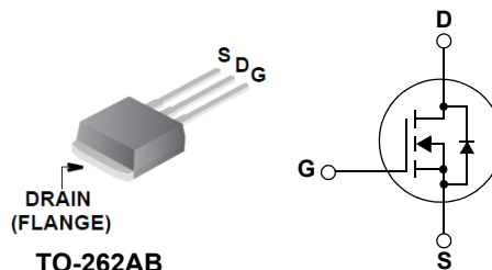
TO-262AB
