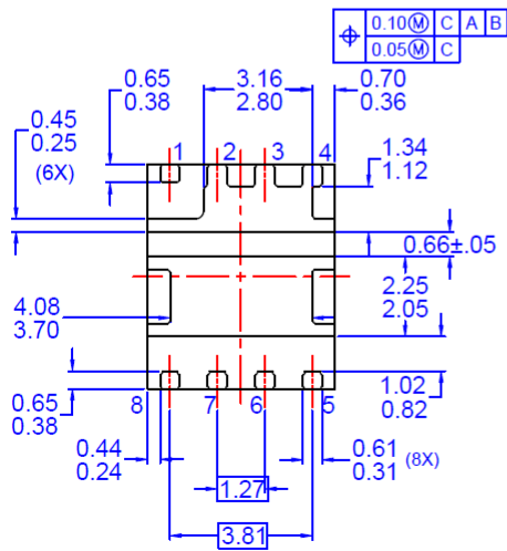
BOTTOM VIEW OPTION - A (SAWN TYPE)
