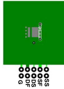
b. 50\text{ }^\circ\text{C}/\text{W} when mounted on a 1\text{ in}^2 pad of 2 oz copper
