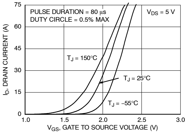
Figure 5. Transfer Characteristics
