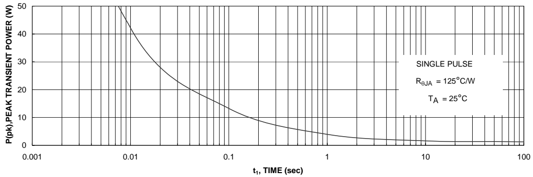
Figure 11 Single Pulse Maximum Power Dissipation.
