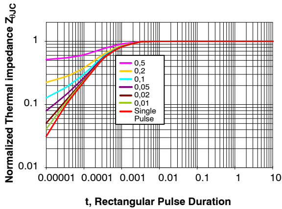
Figure 3. Normalized Maximum Transient Thermal Impedance
