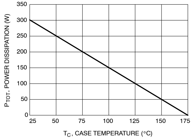
Figure 4. Power Derating
