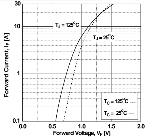
Figure 18. Forward Characteristics
