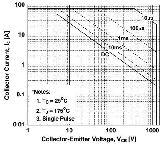
Figure 10. SOA Characteristics
