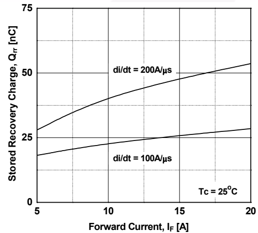
Figure 24. Stored Charge
