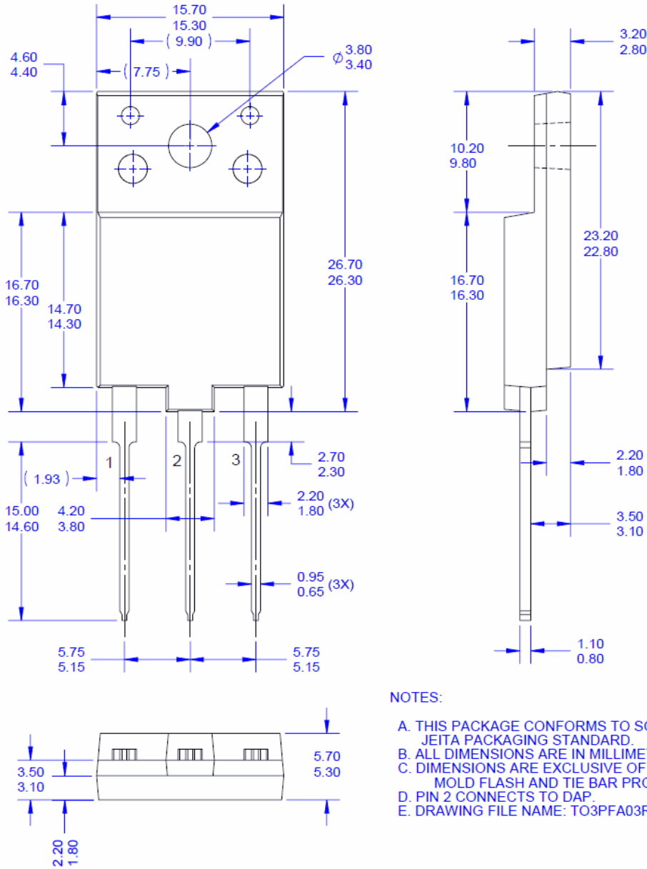
Figure 18. TO3PF,MOLDED,3LD,FULLPACK (AG)
