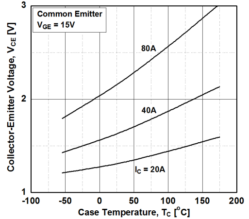
Figure 4. Saturation Voltage vs. Case Temperature at Variant Current
